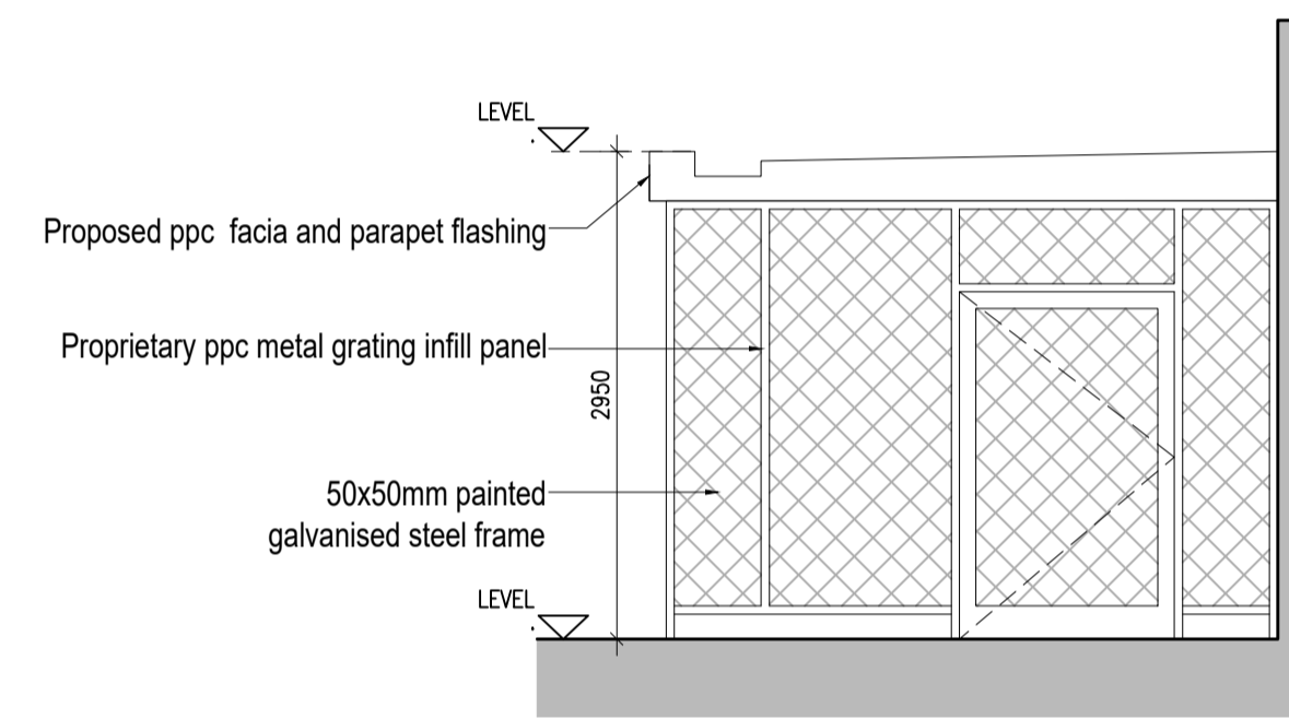
04 Proposed Covered Bicycle Parking Type 3 - Side Elevation 01 P201 1:50@A1
