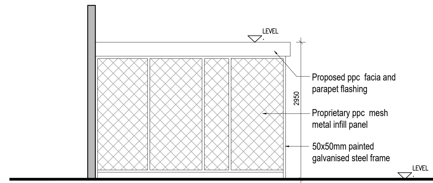
01 Proposed Covered Bicycle Parking Type 3- Front Elevation P201 1:50@A1
