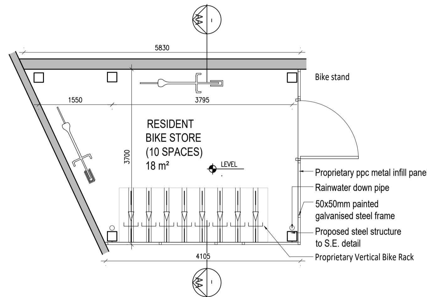
03 Proposed Covered Bicycle Parking Type 3 - Ground Plan P201 1:50@A1
