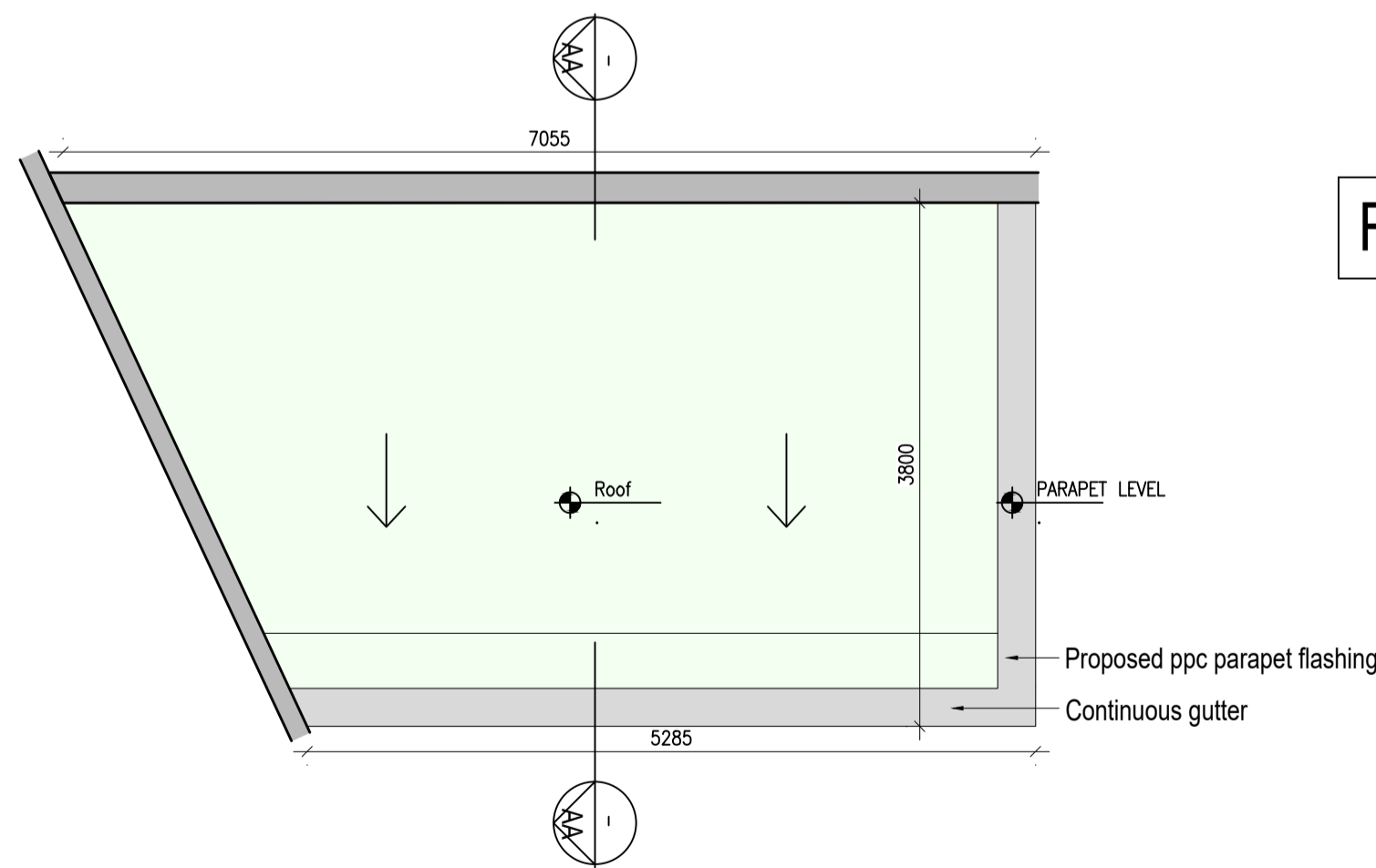
05 Proposed Covered Bicycle Parking Type 3 - Roof Plan P201 1:50@A1
