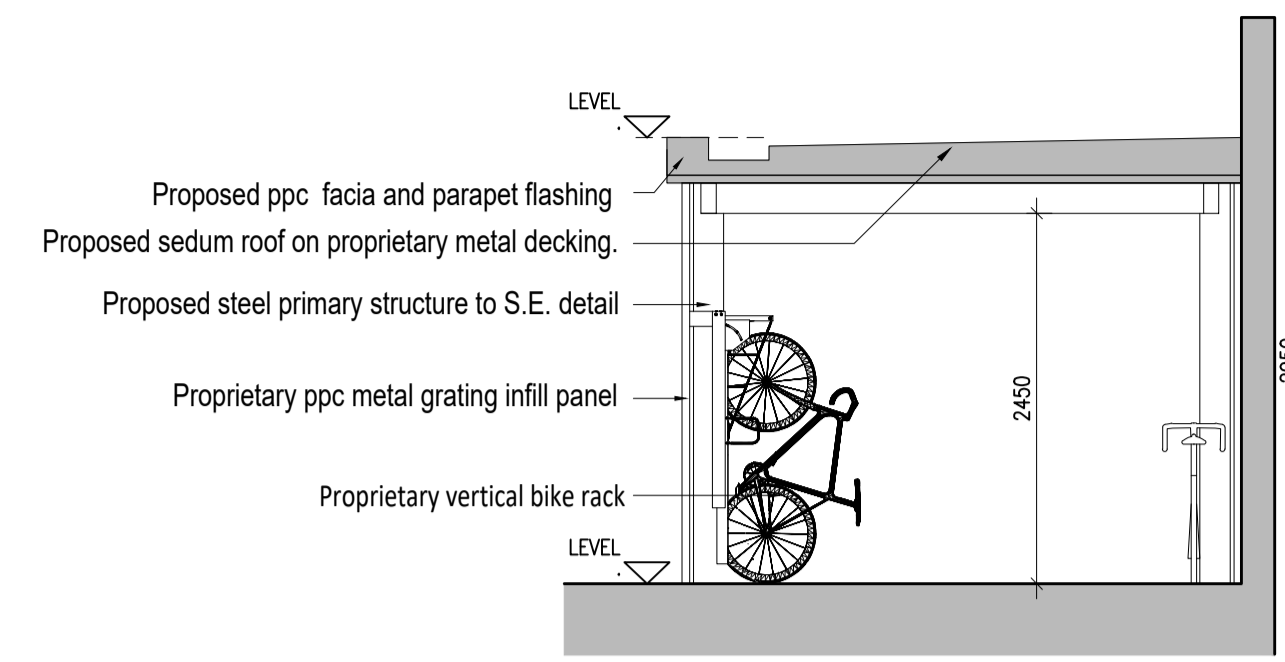
02 Proposed Covered Bicycle Parking Type 3- Section A-A P201 1:50@A1
